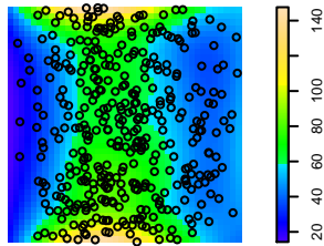
Cubic model: AIC = 27.436
