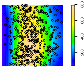
Cubic model: AIC = 27.436
