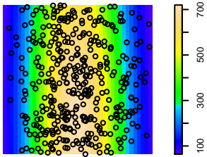
Quadratic model: AIC = 29.499
