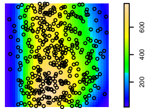
Quartic model: AIC = 32.247
