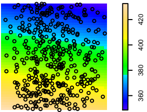
Linear model: AIC = 143.115
