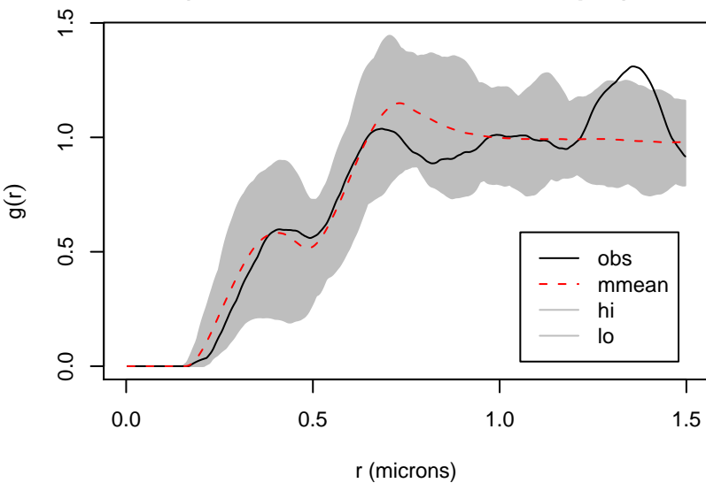
Cell 1 myofibrils PCF (multi-Strauss-hardcore envelopes)
