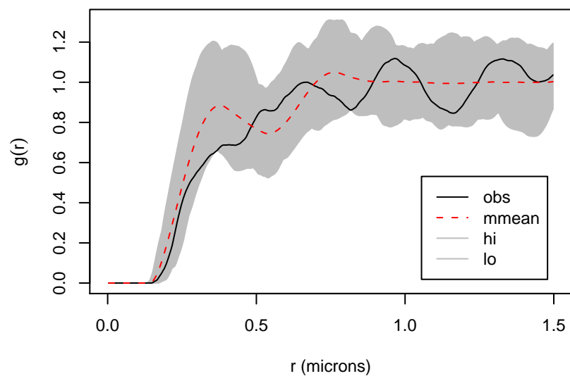
Cell 1 mitochondria PCF (multi-Strauss-hardcore envelopes)
