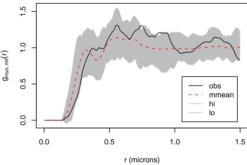
Cell 1 myo-mit cross PCF (multi-Strauss-hardcore envelopes)
