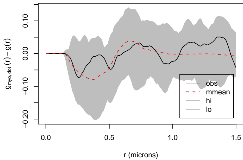
Cell 1 myo-dot PCF (multi-Strauss-hardcore envelopes)
