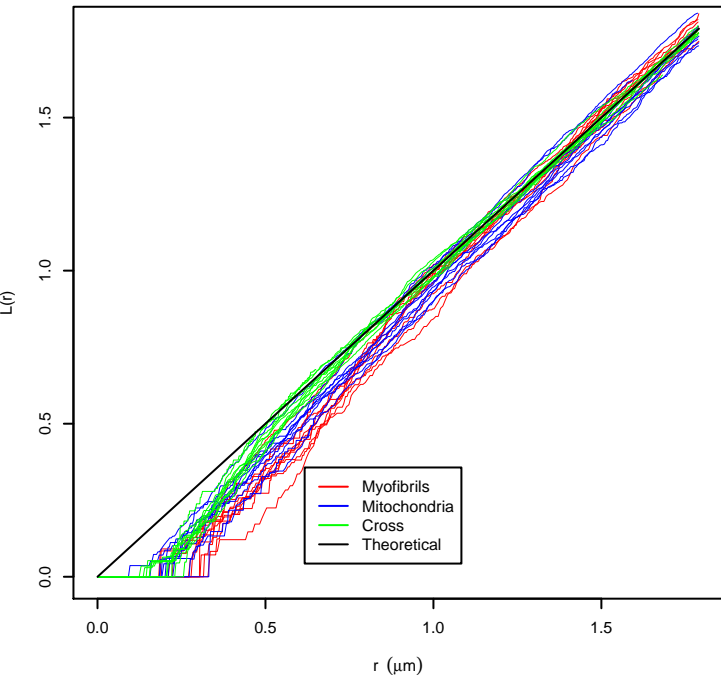
Linearised Pairwise Distances cdf
