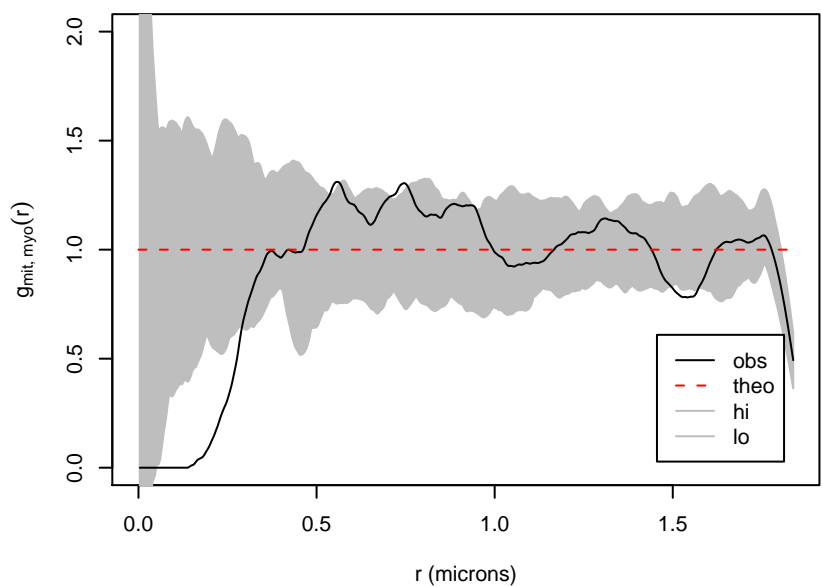
Cell 1 mit-myo cross PCF (Poisson envelopes)
