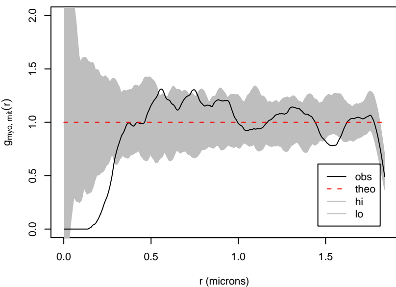
Cell 1 myo-mit cross PCF (Poisson envelopes)
