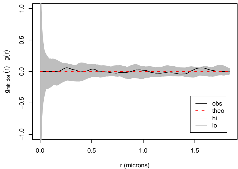
Cell 1 mit-dot PCF (Poisson envelopes)
