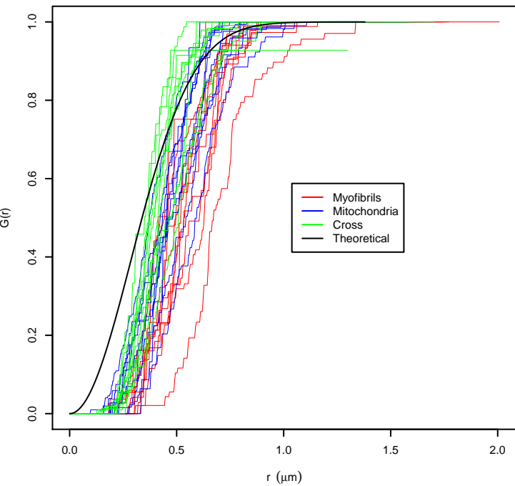
Nearest Neighbour cdf
