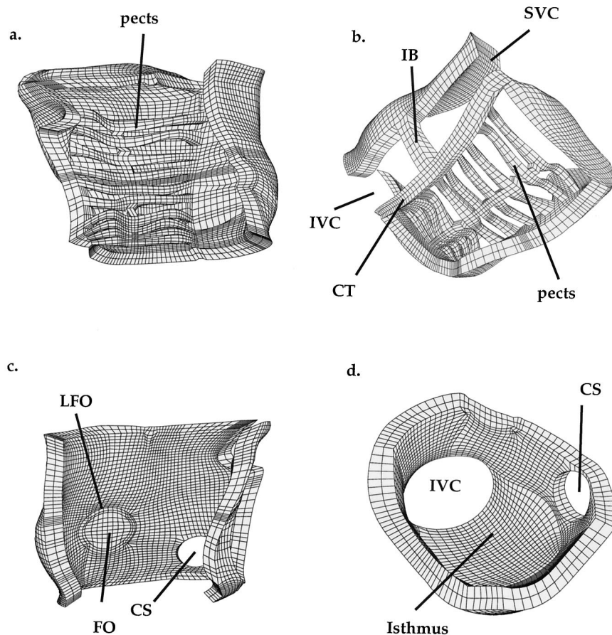
Figure 3. View of the right atrial endocardial structure. Highlighted structures include the pectinates (pectis), crista terminalis (CT), fossa ovalis (FO), coronary sinus (CS), limbus of the fossa ovalis (LFO), superior/inferior vena cava (SVC/IVC), and intercaval bundle (IB).
