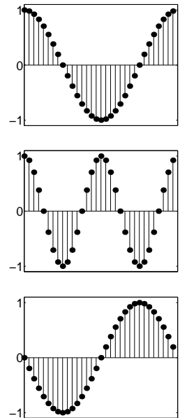
Figure 2.6 f[x] = A \cos[\omega x + \phi]
