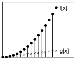
Figure 2.5 g[x] = f[x] \star h[x]
