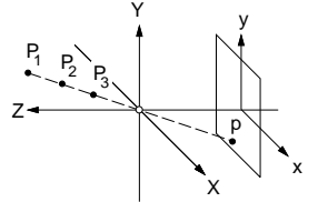
Figure 5.5 Non-invertible projection
