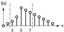
Figure 1.3 Moving Average
