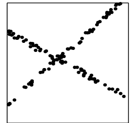
Figure 11.1 Data from two models
