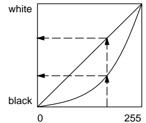
Figure 6.1 Lookup table
