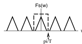
Figure 3.5 Reconstruction
