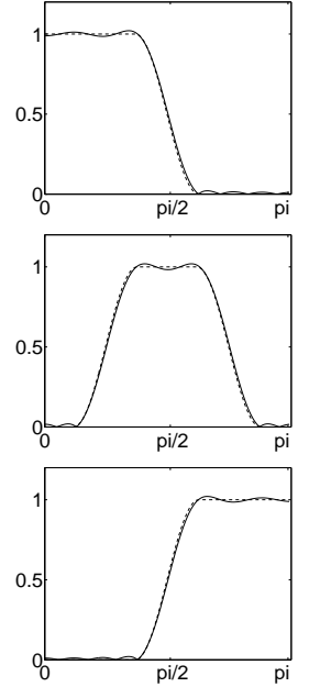
Figure 4.4 Least-squares: lowpass, bandpass, and highpass
