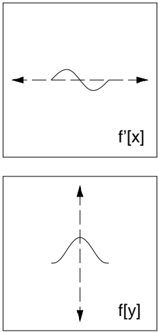
Figure 7.6 Horizontal partial differentiation
