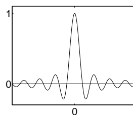
Figure 3.6 Ideal sinc
