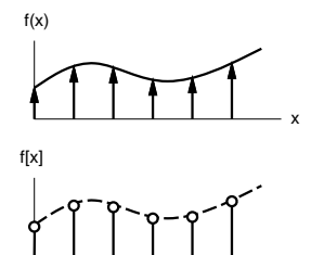
Figure 3.2 Sampling: space
