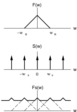
Figure 3.4 Sampling: aliasing
