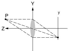
Figure 5.4 Thin lens
