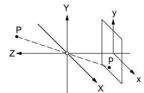
Figure 5.2 Perspective projection
