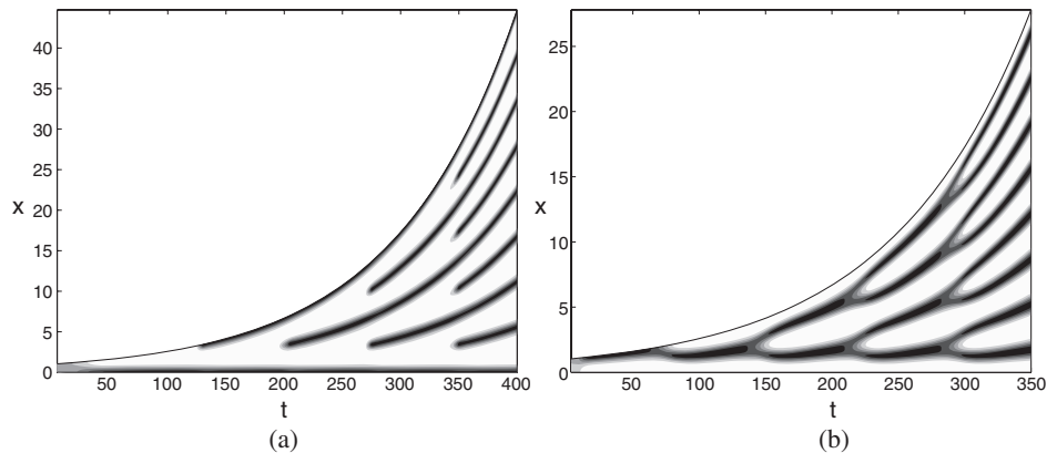
Figure 1. Patterns in the activator v(x, t) obtained on the uniformly growing domain. For domain expansion the patterns change regularly through mode doubling behaviour: (a) Gierer–Meinhardt kinetics, where f(u, v) = v^2 - u and g(u, v) = v^2/u - 0.5v + 0.1 , showing regular insertion of new activator peaks and (b) Schnakenberg kinetics, where f(u, v) = 0.9 - uv^2 and g(u, v) = 0.1 + uv^2 - v , showing peak splitting. In both cases d = 0.025 , \gamma_0 = 1.0 and S = \rho = 0.01 . Numerical solutions are computed using the NAG library routine DO3PCF. The grey-scale is from low (white) to high (black) concentration.
