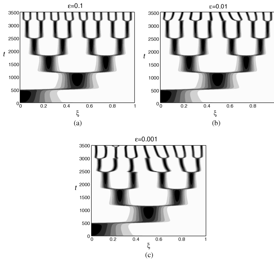
Figure 7. Pattern formation with nonuniform domain growth: as \varepsilon is reduced solutions resemble the piecewise uniform case shown in Fig. 4(a). Here we plot numerical solutions for the activator v(\xi, t) with the tanh function for the domain growth and \rho_1 = 0.001 , \rho_2 = 0.0011 and \Theta = 0.5 . The initial domain length \gamma_0 = 1 and we plot solutions for (a) \varepsilon = 0.1 ; (b) \varepsilon = 0.01 and (c) \varepsilon = 0.001 giving successively closer approximations to the piecewise uniform case.
