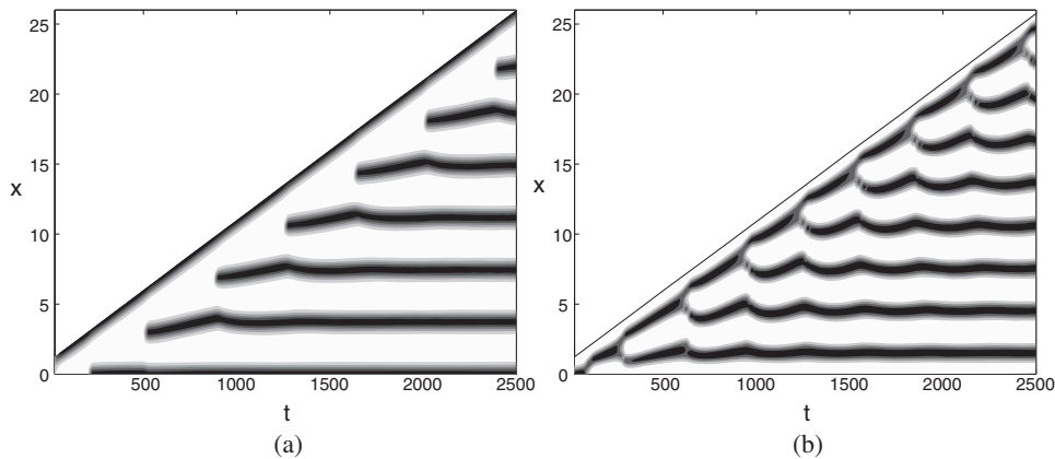
Figure 2. Patterns in the activator concentration obtained under apical growth for (a) Gierer–Meinhardt kinetics showing insertion of new activator peaks near the moving boundary and (b) Schnakenberg kinetics showing splitting of the activator peak proximal to the boundary. Kinetic functions and parameters as for Fig. 1 with S_{\text{tip}} = 0.01/\delta , i.e. r(t) = 1 + 0.01t . Grey-scale is from low (white) to high (black) concentration.
