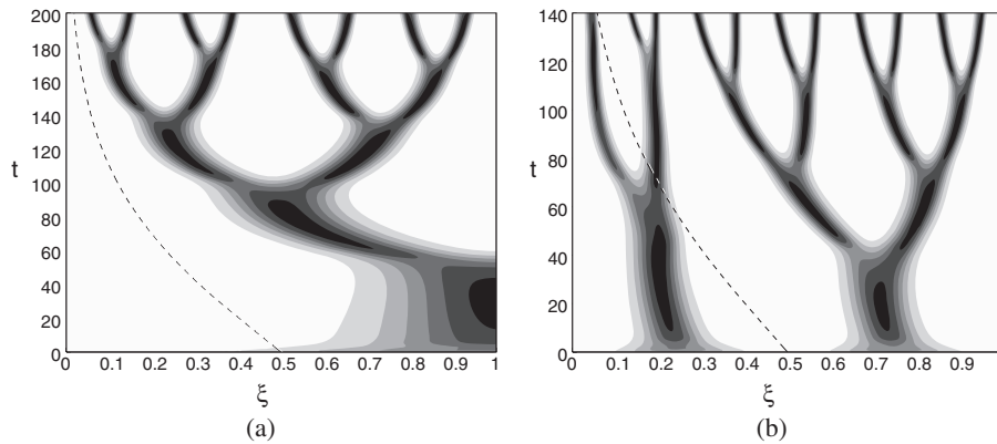
Figure 5. Pattern sequences generated from larger initial domains. The figure shows the activator v(\xi, t) for piecewise uniform domain growth with \rho_1 = 0.0, \rho_2 = 0.02 and (a) \gamma_0 = 1.0 so that the initial mode m = 1 and (b) with \gamma_0 = 20.0 where the initial pattern is mode m = 4 . Other remarks as for Fig. 3.
