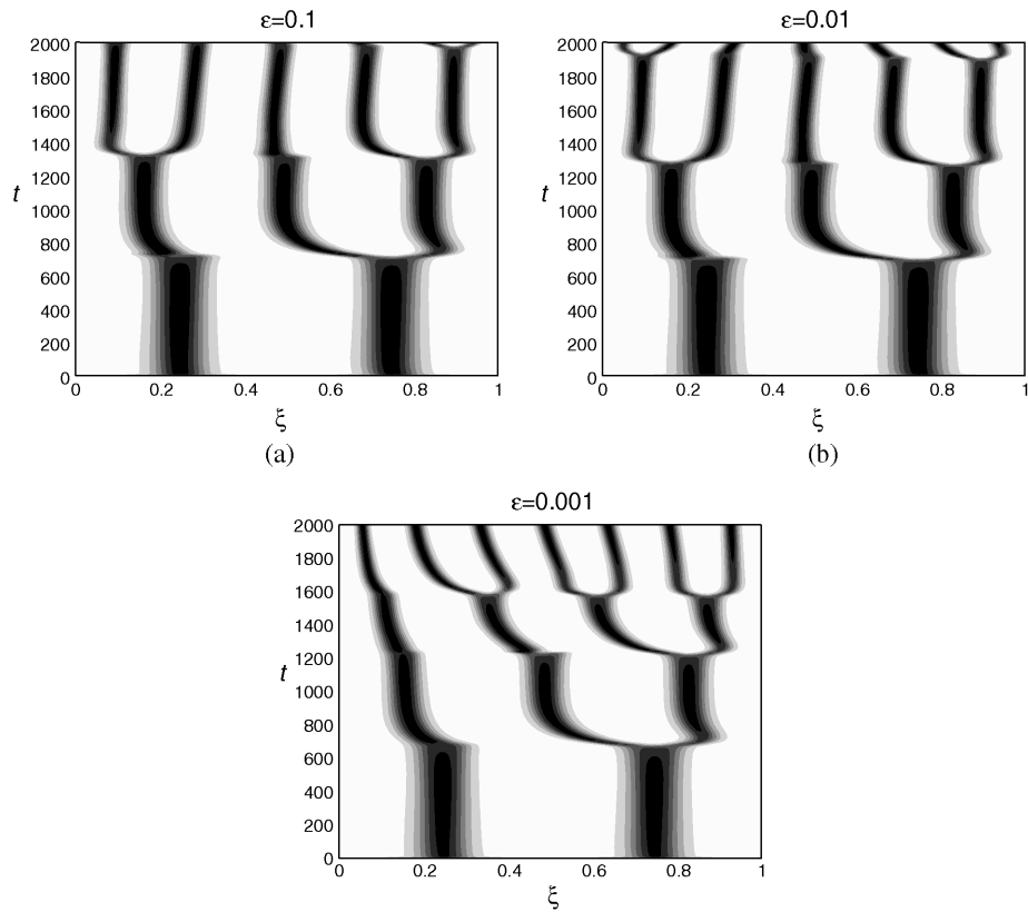
Figure 8. Pattern formation under nonuniform domain growth for larger initial domains. Numerical solutions are shown for the activator v(\xi, t) with the tanh function for the domain growth and \rho_1 = 0 , \rho_2 = 0.001 and \Theta = 0.5 . The initial domain length is \gamma_0 = 20 and we plot (a) \varepsilon = 0.1 , (b) \varepsilon = 0.01 and (c) \varepsilon = 0.001 .
