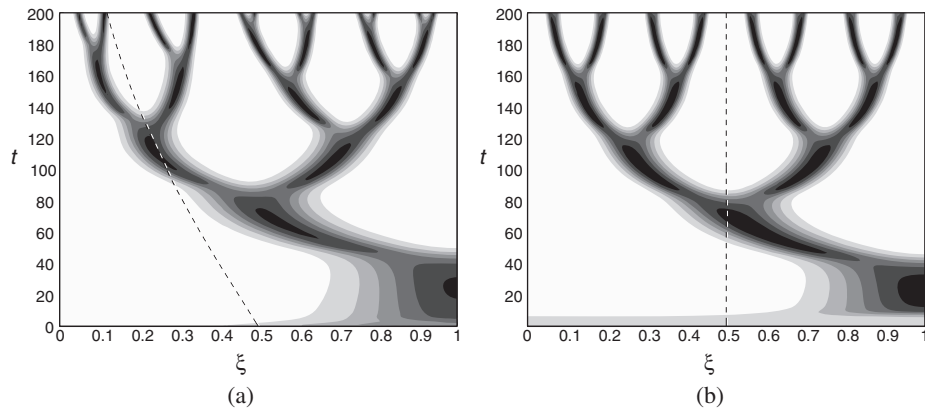
Figure 3. Asymmetric peak splitting for piecewise uniform domain growth, with Schnakenberg kinetics. Numerical solutions v(\xi, t) are shown on the unit interval for (a) piecewise uniform domain growth with \rho_1 = 0.01 , \rho_2 = 0.02 and \gamma_0 = 1 and (b) uniform domain growth with \rho = 0.017 and \gamma_0 = 1 giving (approximately) the same dimensional domain length at time t = 200 . Shading is 0 (white) to 4 (black). In this and subsequent figures the initial conditions were chosen such that a right-hand boundary peak is first generated. Further numerical simulations (data not shown) demonstrate that the pattern sequence and asymmetry are the same for an initial peak located on the left-hand boundary. For ease of comparison the faster-growing sub-domain is on the right-hand side.
