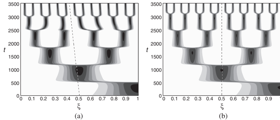
Figure 4. Missing peaks for piecewise uniform domain growth. The figure shows numerical solutions for the activator v(\xi, t) for (a) piecewise uniform domain growth with \rho_1 = 0.001 , \rho_2 = 0.0011 and \gamma_0 = 1 and (b) uniform domain growth with \rho = 0.00105 and \gamma_0 = 1 giving (approximately) the same dimensional domain length at time t = 3500 . Other remarks as for Fig. 3.
