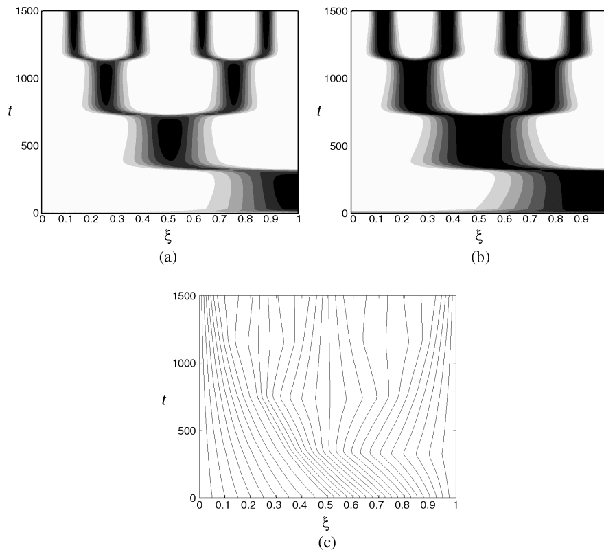
Figure 9. Pattern formation with reactant-controlled domain growth. We plot (a) the activator (the ‘growth factor’) on the transformed domain and (b) the local strain rate for Schnakenberg kinetics and with \gamma_0 = 1 , d = 0.01 , \rho = 0.005 , \kappa = 1 and m = 1 . In (c) the flow lines, \Gamma(X, t)/\Gamma(1, t) , are plotted, i.e. trajectories of particles initially separated at regular intervals in X . For clarity twice as many points are taken in the second half as in the first half of the interval X \in [0, 1] . We have taken \alpha = 0 although we have found no qualitative change to the results for small non-zero \alpha . The numerical mesh has 1000 space points and no change to the solution is found by halving the mesh size. Numerical solutions were also computed with sigmoidal response functions for higher cooperativity, m > 1 , and for other values of \kappa , giving qualitatively similar results.
