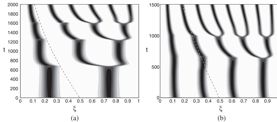
Figure 6. Pattern sequences generated from larger initial domains. Numerical solutions for activator v(\xi, t) are shown for piecewise uniform domain growth with \rho_1 = 0.0 , \rho_2 = 0.001 and (a) \gamma_0 = 20.0 so that the initial mode to grow is mode m = 4 and (b) \gamma_0 = 80.0 where the initial pattern is m = 8 . Other remarks as for Fig. 3.
